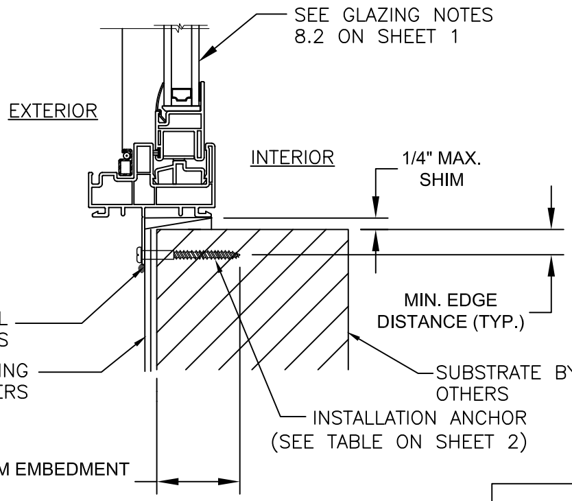
A 4 ANCHOR DETAIL NAILING FIN FRAME SILL
