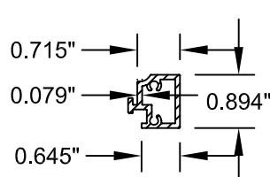
⑫ INTERLOCK/LIFT RAIL ALUM. REINF.-612429
