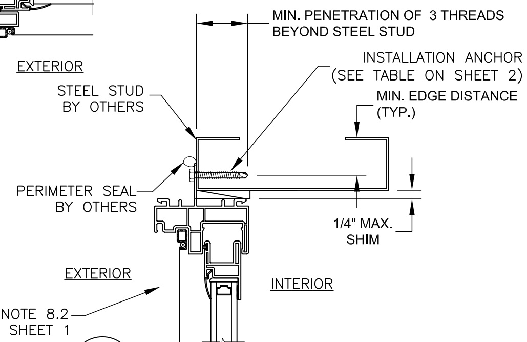
E 4 VERTICAL SECTION STEEL STUD STRUCTURE NAIL FIN INSTALLATION HEAD SHOWN, SILL & JAMBS SIMILAR
