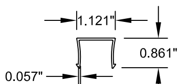
③ STOP/COVER UPVC-500124
