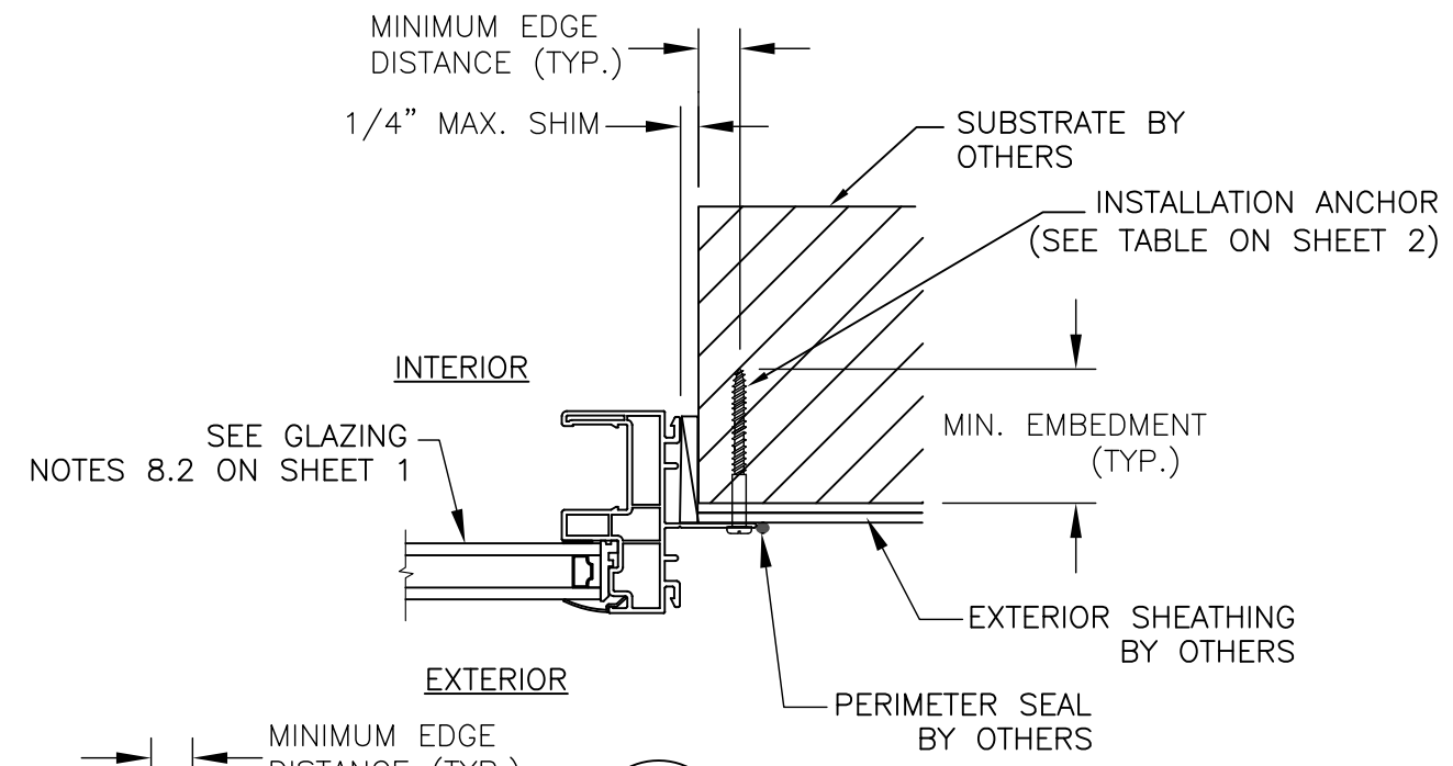
C 4 ANCHOR DETAIL NAILING FIN STATIONARY JAMB
