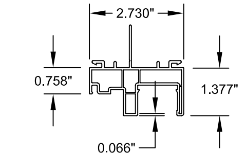
① FRAME WITH NAIL FIN EQUAL LEG UPVC-606004
