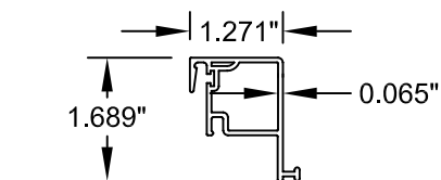
④ INTERLOCK/LIFT RAIL SASH UPVC-606005
