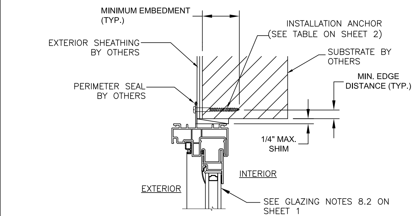
B 4 ANCHOR DETAIL NAILING FIN FRAME HEAD
