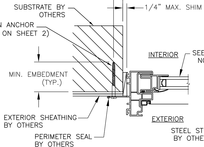
D 4 ANCHOR DETAIL NAILING FIN OPERABLE JAMB
