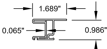
⑤ COMMON SASH UPVC-606007
