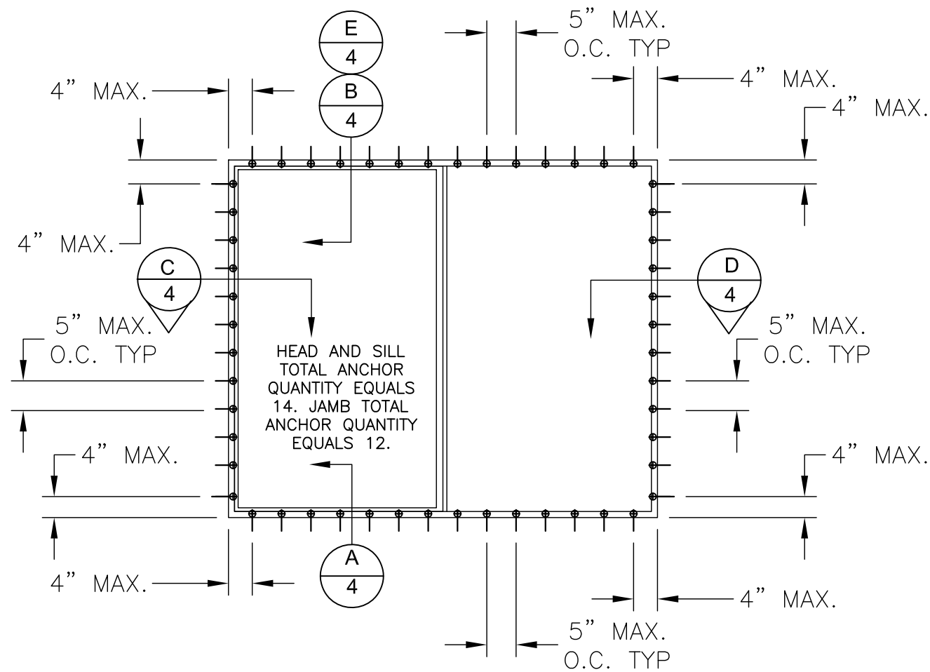
ANCHOR LAYOUT NAILING FIN 72" X 60" INSTALLATION
